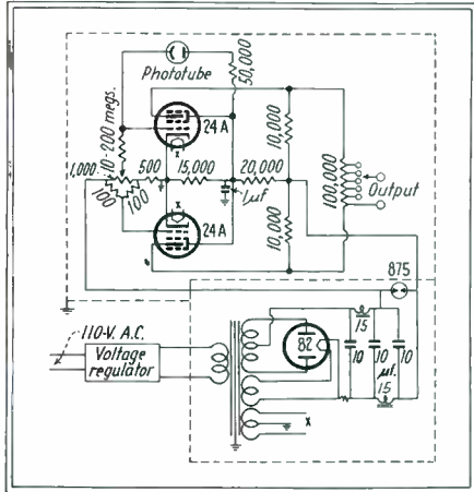
Diagram of bridge-type balanced amplifier
