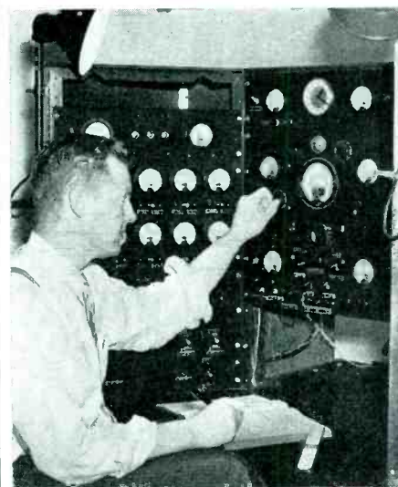
Professor L. N. Ridenour, Jr. of the University of Pennsylvania at the control board of the new 5,000,000-volt electrostatic generator now under construction in the Department of Physics.
