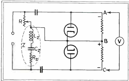
Fig. 2—Circuit to overcome phase difference difficulties
