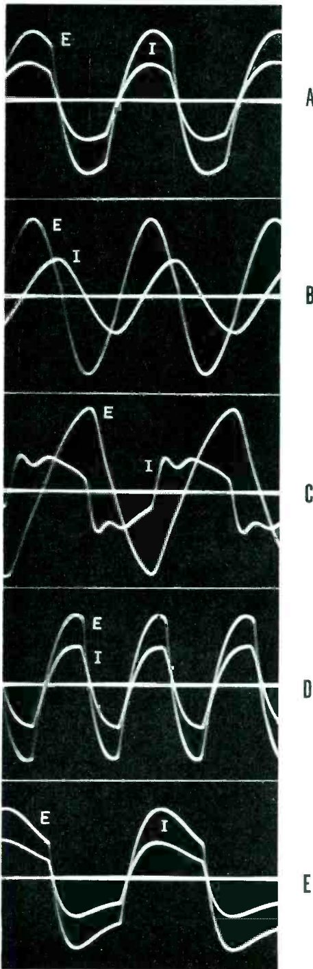
Fig. 7—Input voltage held constant with output voltage and frequency set to normal values at light load and both allowed to vary at will
